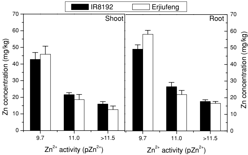
Figure 1. Zinc concentration in the shoots and roots of Zn efficient genotype IR8192 and Zn inefficient genotype Erjiufeng grown at different Zn 2+ activities.
